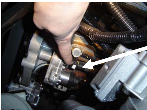
Step 6 - This is a photo of the OEM quick connect fitting that will be disconnected apart from the pump. Once disconnected, adapt the Fitch 2” male hose to the OEM female feed line & the Fitch 24” female quick connect to the OEM male off the injector pump.
